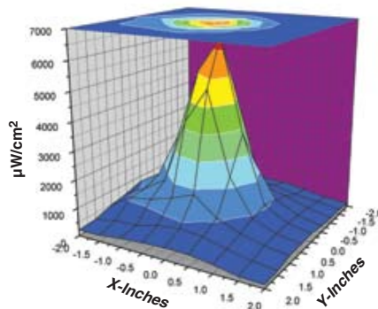
SURFACE CONTOUR PROFILE AT 24 IN (61 CM)
