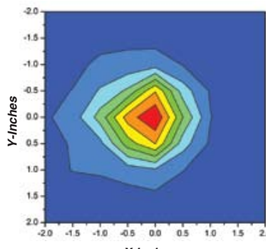
TOP INTENSITY PROFILE AT 24 IN (61 CM)
