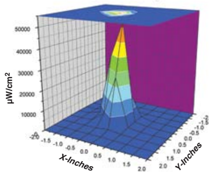
SURFACE CONTOUR PROFILE AT 6 IN (15 CM)
