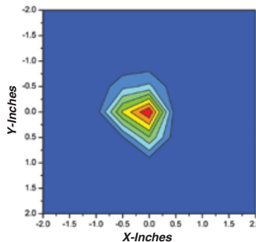
TOP INTENSITY PROFILE AT 6 IN (15 CM)
